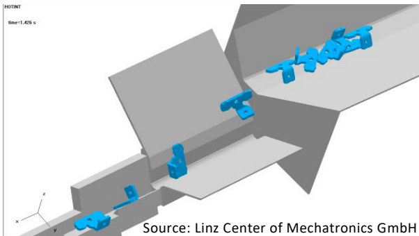
Simulation of the conveying process with several feeding parts in the multibody dynamics tool HOTINT ( https://hotint.lcm.at )
